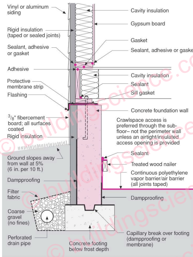
Figure 10 Externally Insulated Concrete Crawl Space with Vinyl or Aluminum Siding Above
